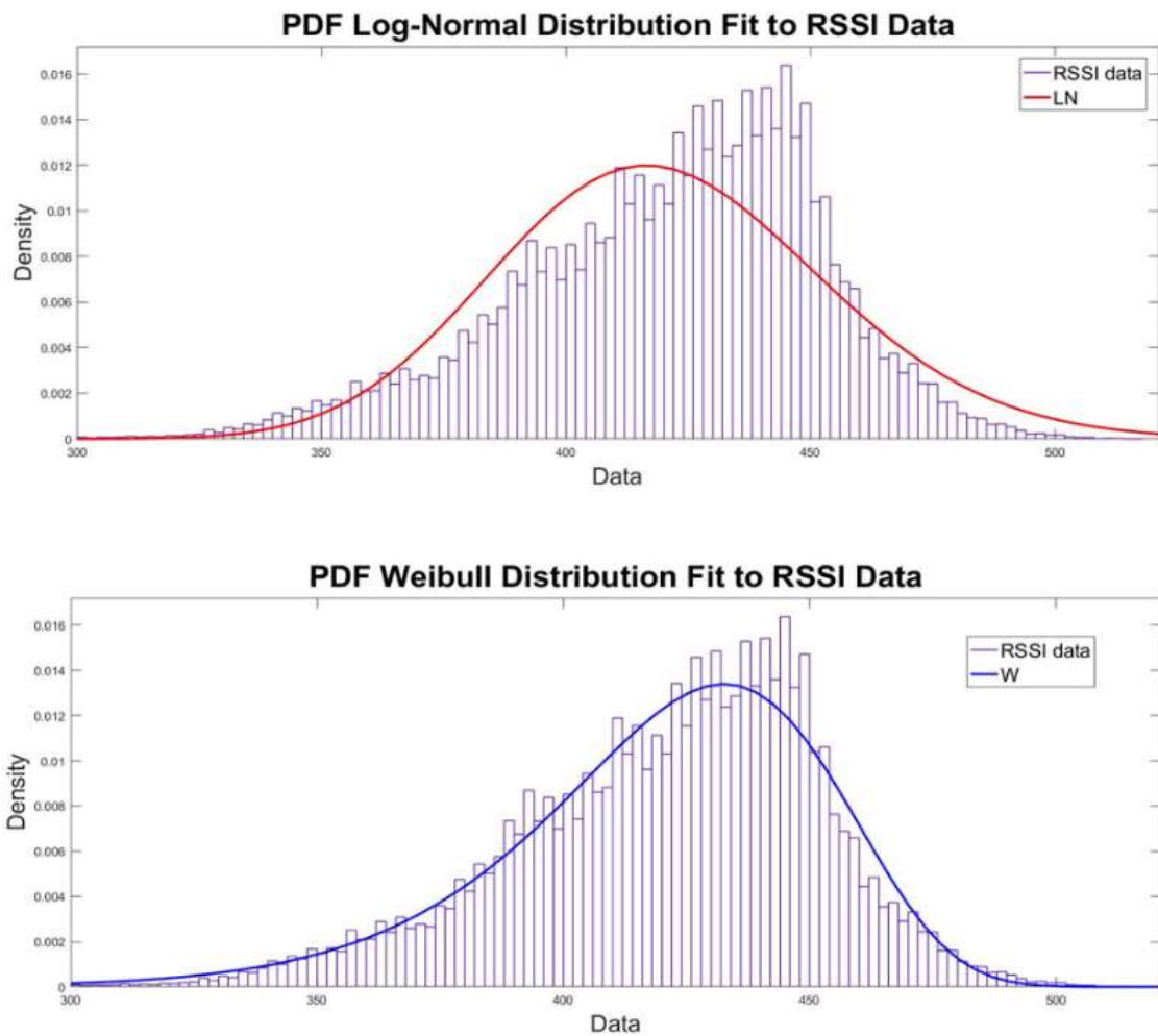
Figure 8.2. Probability density functions fits to RSSI data.
