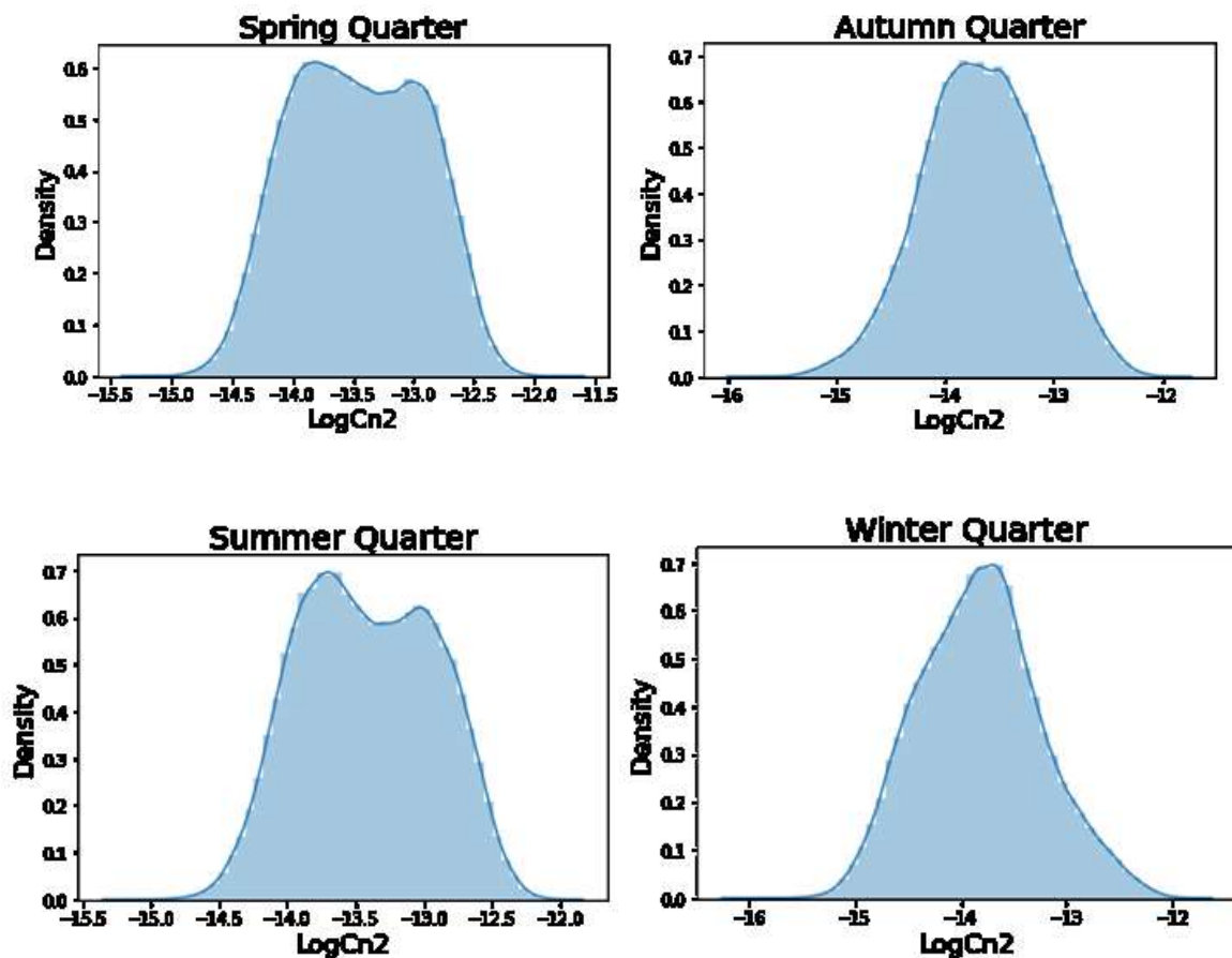
Figure. 7.2. Distribution plots for LogC_n^2 per season.
