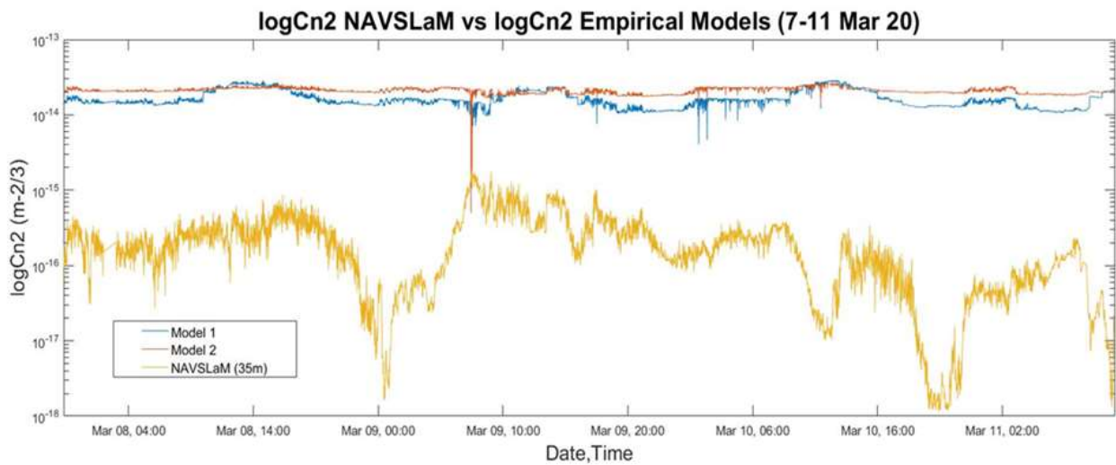
Figure 5.17. Prediction of C_n^2 over the period from 7 to 11 Mar 20. NAVSLaM model (yellow line) as compared to empirical models.
